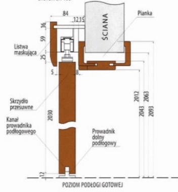
SYSTEM SN 100
