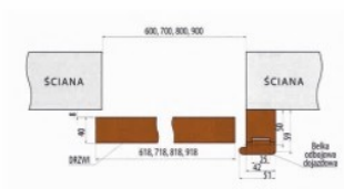
SYSTEM SN 100
